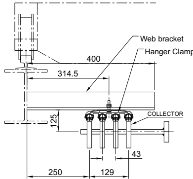
Safe Power - W General Arrangement
