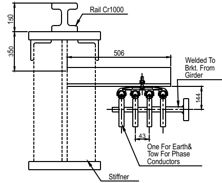
Safe Power - W General Arrangement
