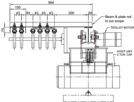
Safe Power - W General Arrangement
