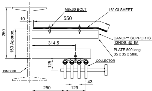
Safe Power - W General Arrangement
