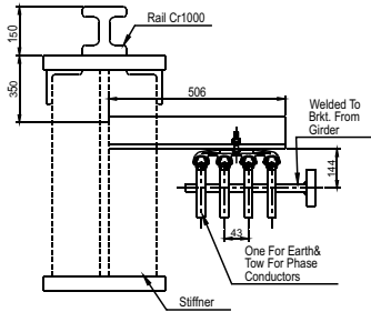
Safe Power - W General Arrangement
