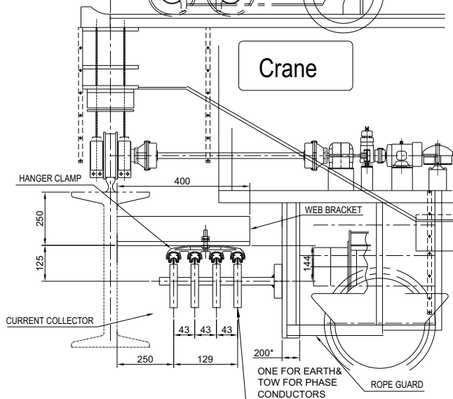
Safe Power - W General Arrangement
